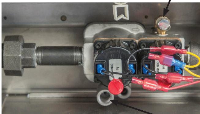
Fig 3.J - 2018 and older, valve design
